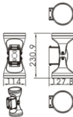
PHBN80002-WL
